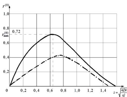
Fig. 1. The dependence of the ratio of the explosive mass of hydrogen to the initial mass from z = \sqrt{4Dt/r_0^2} at the instantaneous release of hydrogen: into oxygen (line), into the air (- . -)
