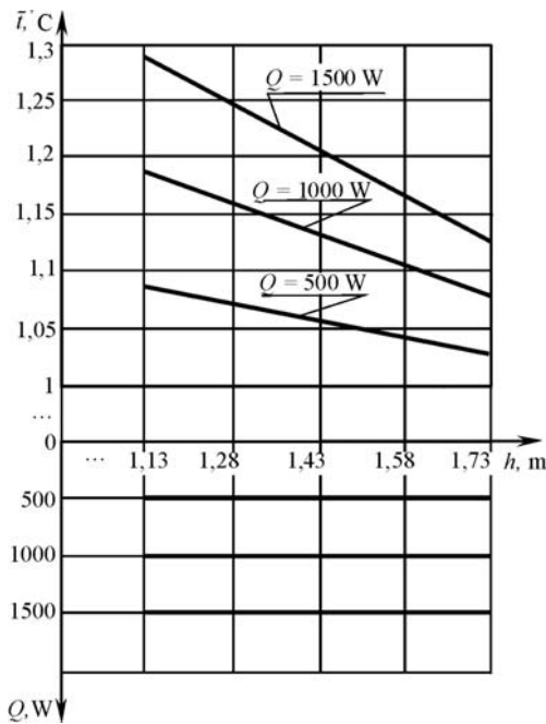
Fig. 7. Surface projections \bar{t} = f(Q, h)
