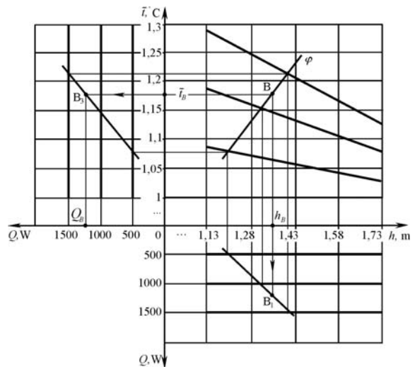
Fig. 9. Definition of the numerical values of parameters h, Q, \bar{t} at any point in the space of premises
