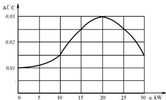
Fig. 5. Excess of relative air temperature on an enabled fan
