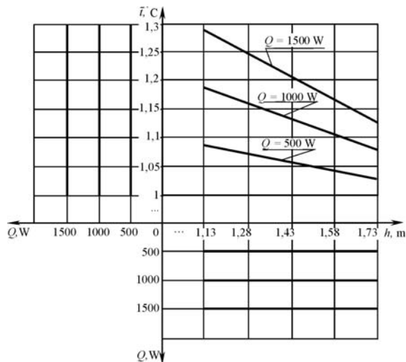
Fig. 8. Setting the surface \bar{t} = f(Q, h) by line frame
