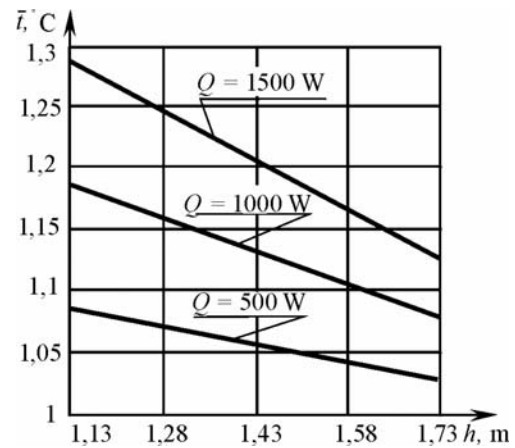
Fig. 6. Influence of height of installation h and thermal power of infrared heater Q to relative air temperature \bar{t} in the service area
