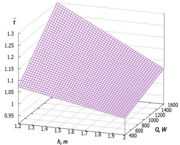
Fig. 11. The surface of temperature in service area
