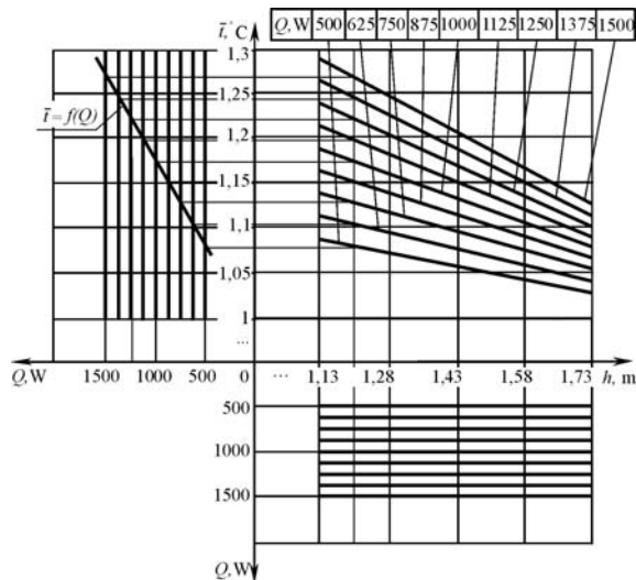
Fig. 10. Construction of the surface frame for nine thermal power values of infrared heater Q
