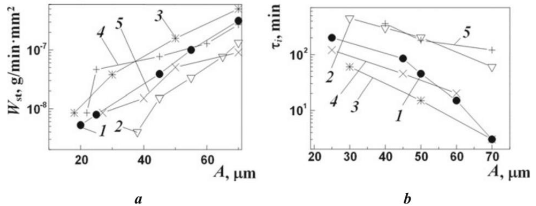
Fig. 7.6 Dependence of the stabilized CED rate ( a ) and the incubation time ( b ) on the amplitude of testing 40Kh steel samples after technological processing methods: (1, 1) normalization, (2, 2) hardening with low tempering (200 °C), (3, 3) VCH ( m = 3.5 kg, \tau = 20 min), (4, 4) VCH ( m = 4.5 kg, \tau = 28 min), and (5, 5) VCH ( m = 7.5 kg, \tau = 28 min)
