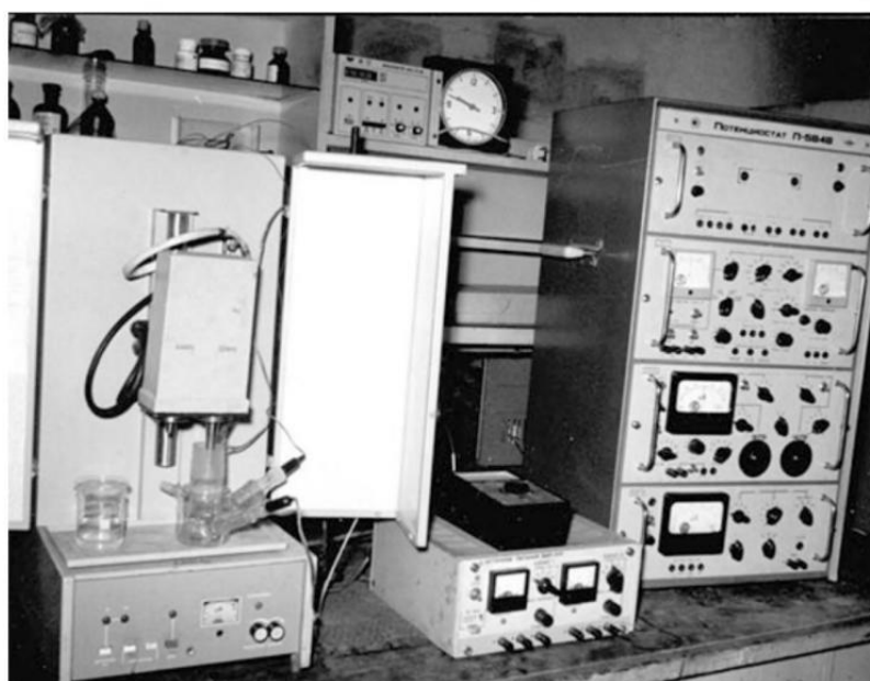
Fig. 7.2 Magnetostrictive unit of CED resistance investigation
