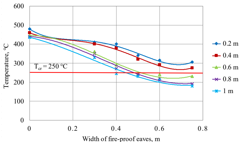
Fig. 13. Dependence plot of changes in temperature values depending on the width of a fire-proof eaves and the height of a window interfloor partition
