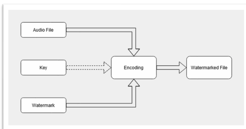
Figure 1 – Embedding process
