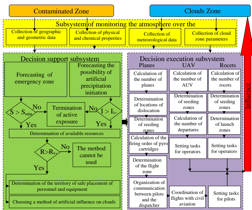
Figure 9. Algorithm for the implementation of the method of liquidation of the consequences of large-scale emergencies of a natural and man-made nature with the release of hazardous substances into the atmosphere
