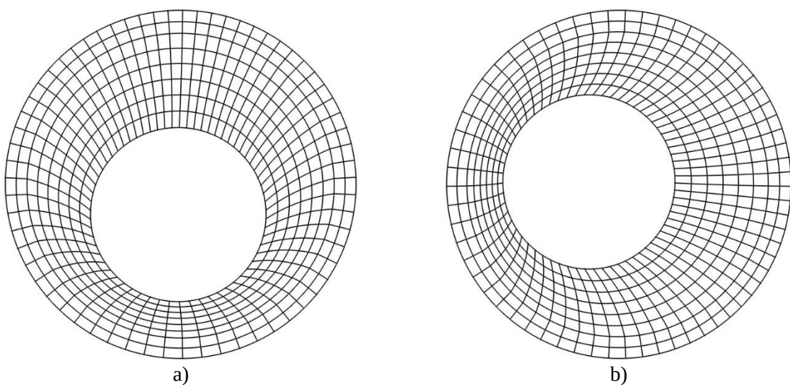
Figure 2 – The second and third multiple eigenmodes of the circular element of agricultural transportation device
