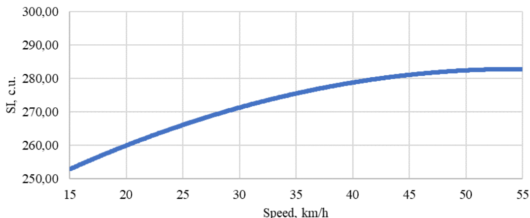
Figure 2 – The impact of the vehicle's speed on the stress index of the driver in urban conditions
