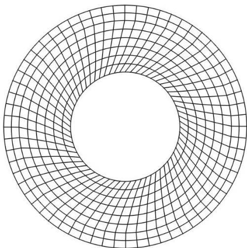
Figure 1 – The first eigenmode of the circular element of agricultural transportation device
