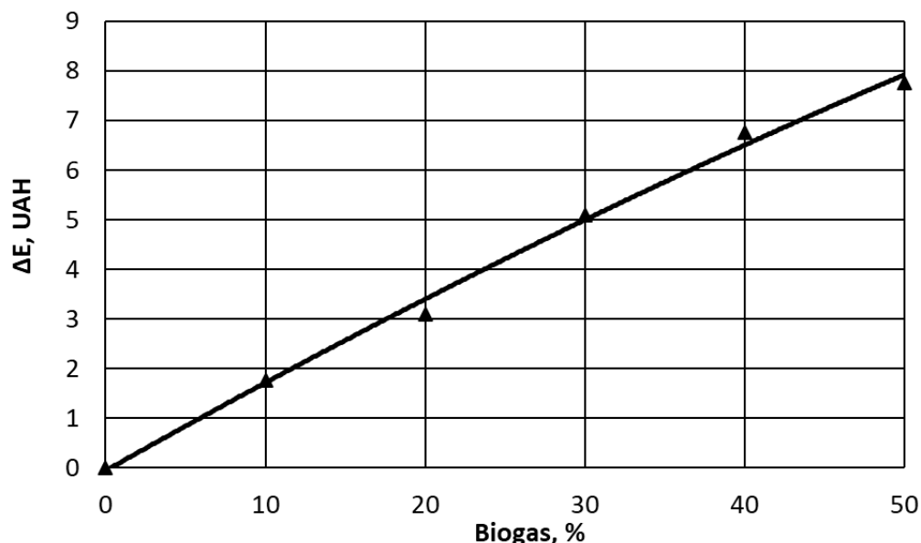
Figure 2 – Dependence of the efficiency of using equivalent fuels based on commercial gasoline on the biogas content in them
