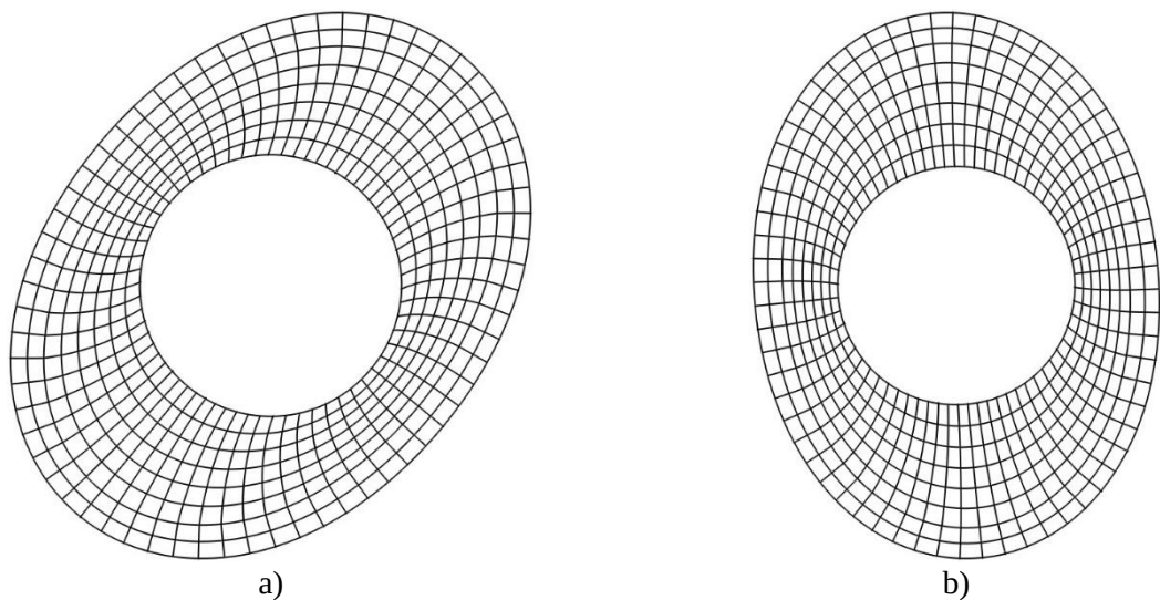
Figure 3 – The fourth and fifth multiple eigenmodes of the circular element of agricultural transportation device
