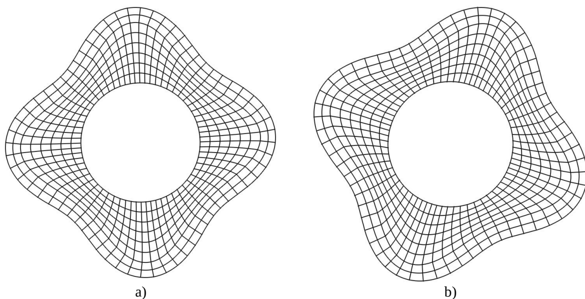
Figure 5 – The eighth and ninth multiple eigenmodes of the circular element of agricultural transportation device
