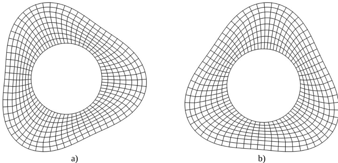
Figure 4 – The sixth and seventh multiple eigenmodes of the circular element of agricultural transportation device
