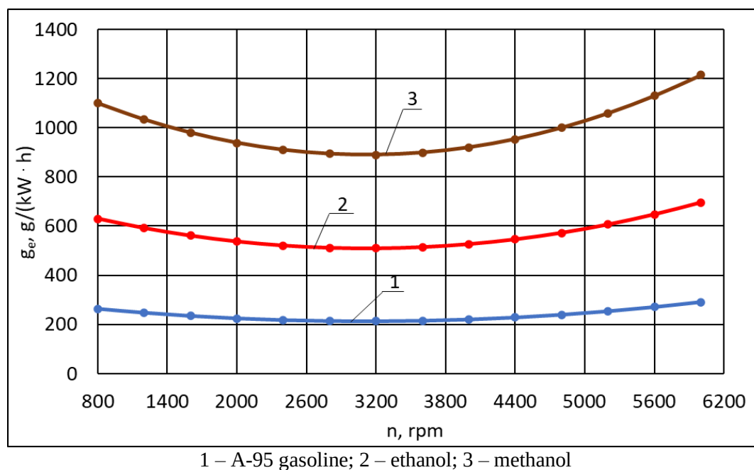
Figure 1 – Experimental graphical dependence of specific effective fuel consumption g_e when using different types of fuel on the Peugeot 3008 engine
