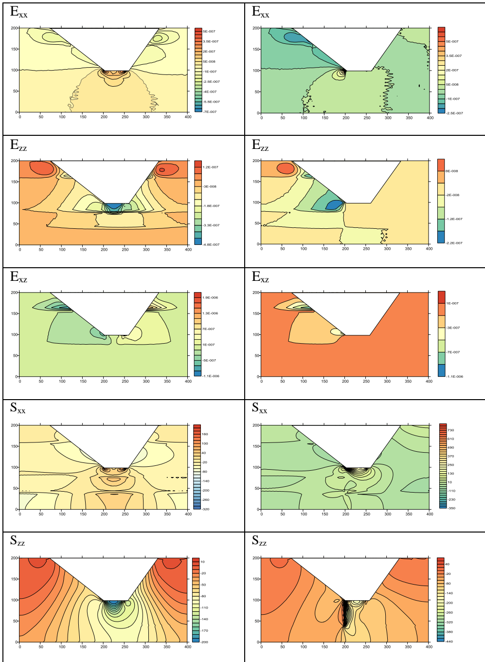
Fig.4. Distribution of strain ( E_{xx} , E_{zz} , E_{xz} ) and stress ( S_{xx} , S_{zz} ) in a "contour map", derived numerical values on the edge of the water-shore shown as a column on the right of each graph. The influence of hydrostatic pressure is taken in to account
