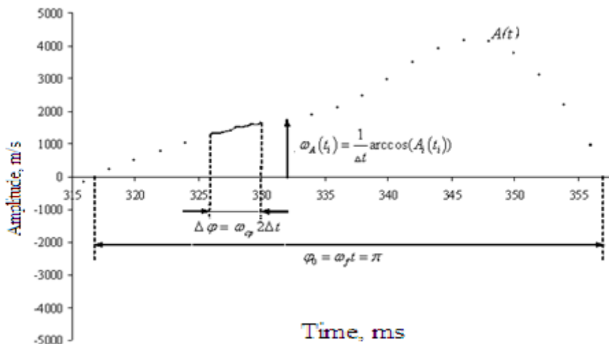
Fig.5 Fragment of the seismogram (dependent from time) and meaning of frequencies instantaneous, transfer, averaged
