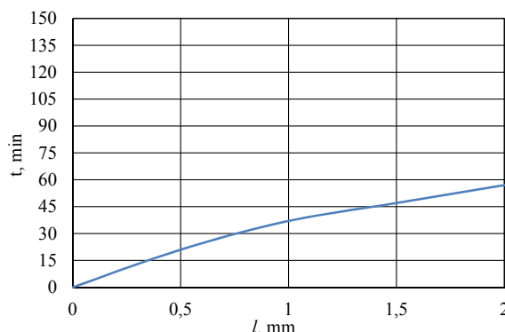
Fig. 2. Dependence of time needed to reach a critical temperature on the coating’s thickness for a metallic plate
