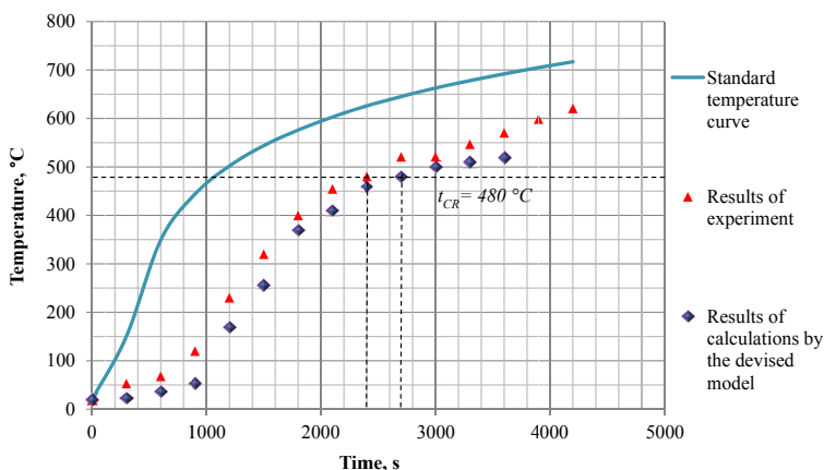
Fig. 1. Results of analysis of experimental measurements of temperature and its obtained values in line with the devised model, depending on time (coating’s thickness is 0.8 mm)
