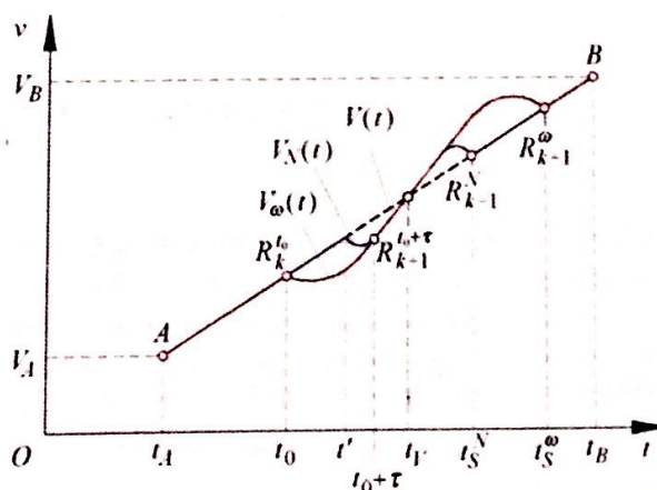
Fig. 1. Fragments of the program of movement of the car
