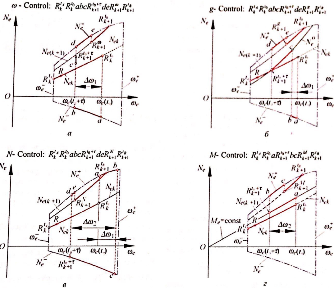
Fig. 2. Combination of operating modes of the engine and a step-by-step transmission of the car
