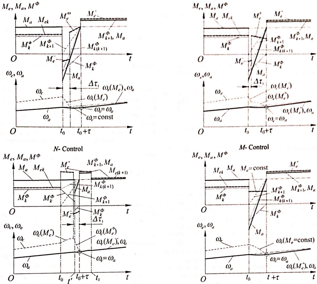
Fig. 5. Fragments of programs for changing the modes of operation of the engine and frictions
