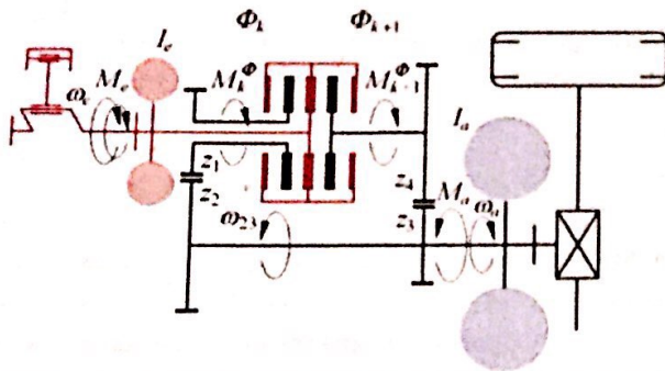
Fig. 3. The scheme of combination in the transmission of a car of two levels, one of which - the direct transmission
