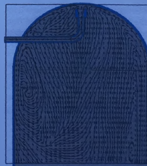
Fig. 3. Trajectories of gas motion inside the body of the damping attachment
