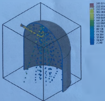
Fig. 4. Trajectories of solid particles motion inside a damping attachment
