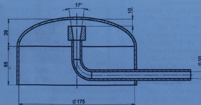
Fig. 5. Estimated model of a damping attachment with an elliptical top
