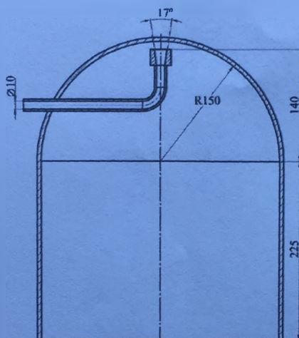
Fig. 1. Structural diagram of the damping attachment for a fire-extinguishing powder feed (estimated model)
