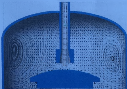
Fig. 11. Trajectories of gas motion inside the discharge nozzle damping attachment's body with an additional mirror
