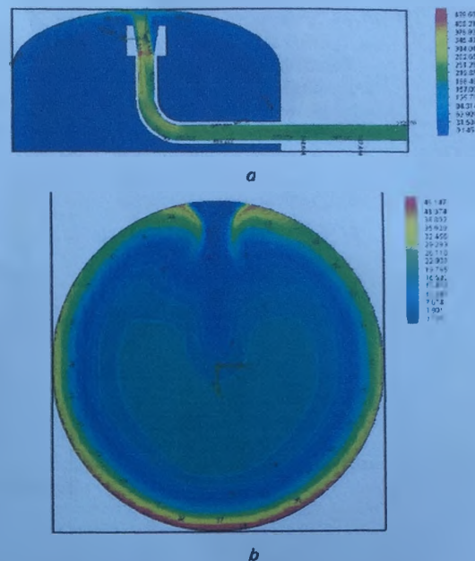
Fig. 6. Chromogram of gas leakage: a – vertical symmetrical cross-section; b – horizontal cross-section at the outlet
