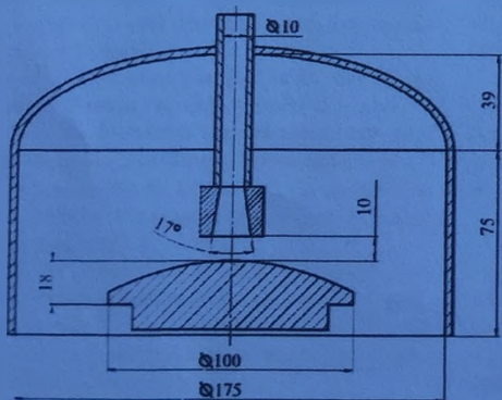
Fig. 9. Estimated model of a damping attachment with an elliptical top and an additional parabolic mirror
