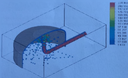
Fig. 8. Trajectories of solid particles motion inside a discharge nozzle damping attachment's body
