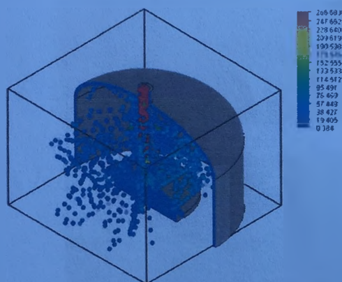
Fig. 12. Trajectories of solid particles motion inside the discharge nozzle damping attachment's body with an additional mirror
